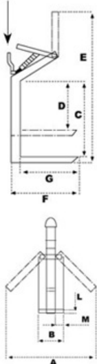
Adjustment handwheel
